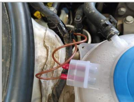
Engine Wiring
