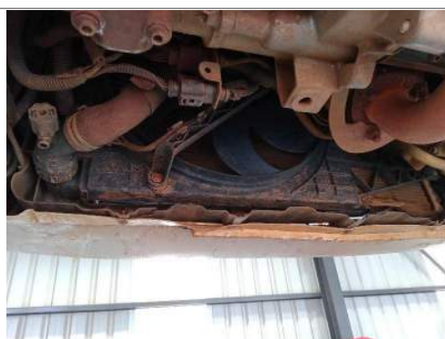
Radiator Cradle
