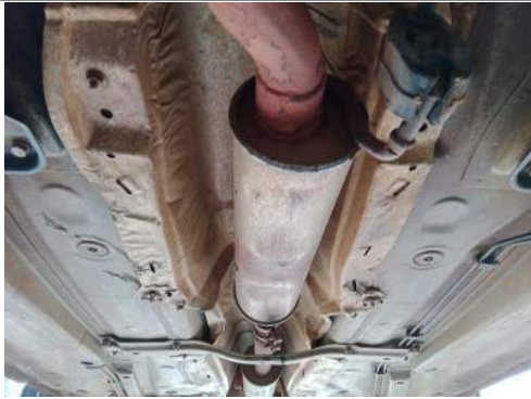
Belly plates
