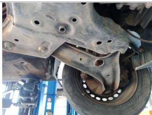
Control Arm(s) Front Axle Left
