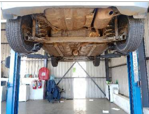
Undercarriage rear.
