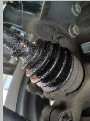
CV Joint(s) Boot(s) Front Right (inner/outer)
